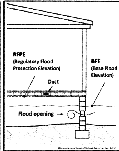
Figure 5: Internally flooded enclosed area.
